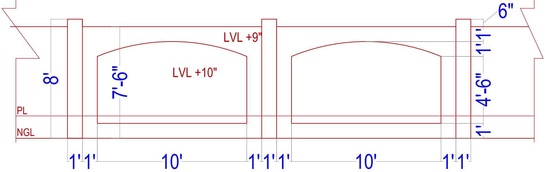
WALL ELEVATION
